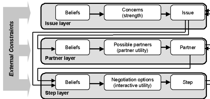
Fig. 2. The IPS framework.
